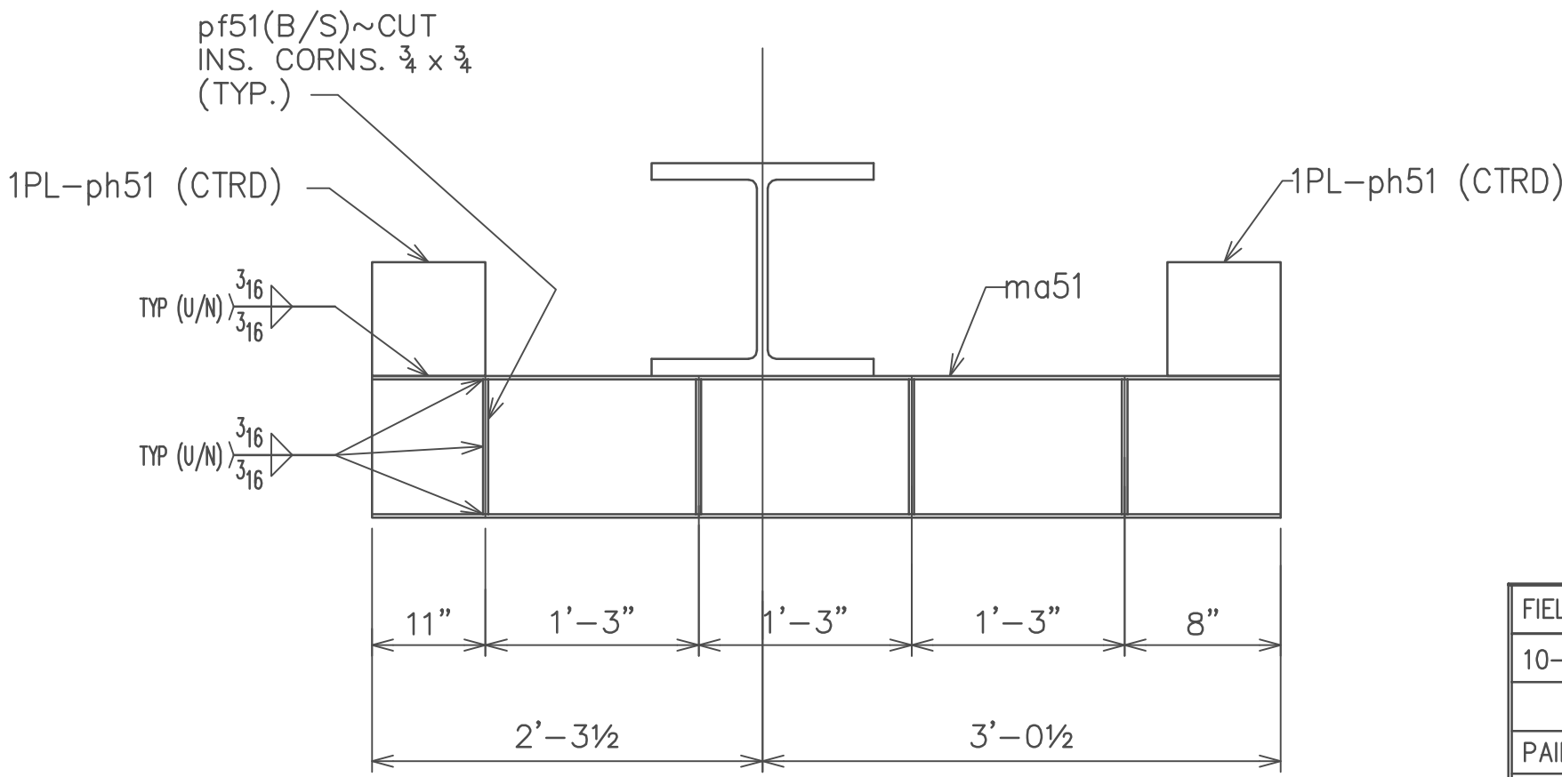
SECTION D
