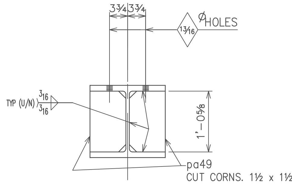
SECTION A
