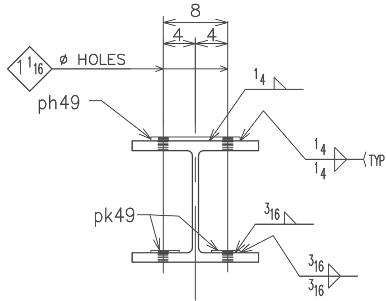
SECTION C
