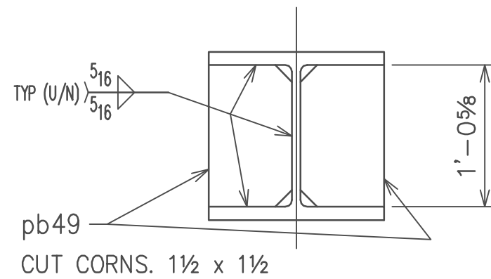
SECTION B
