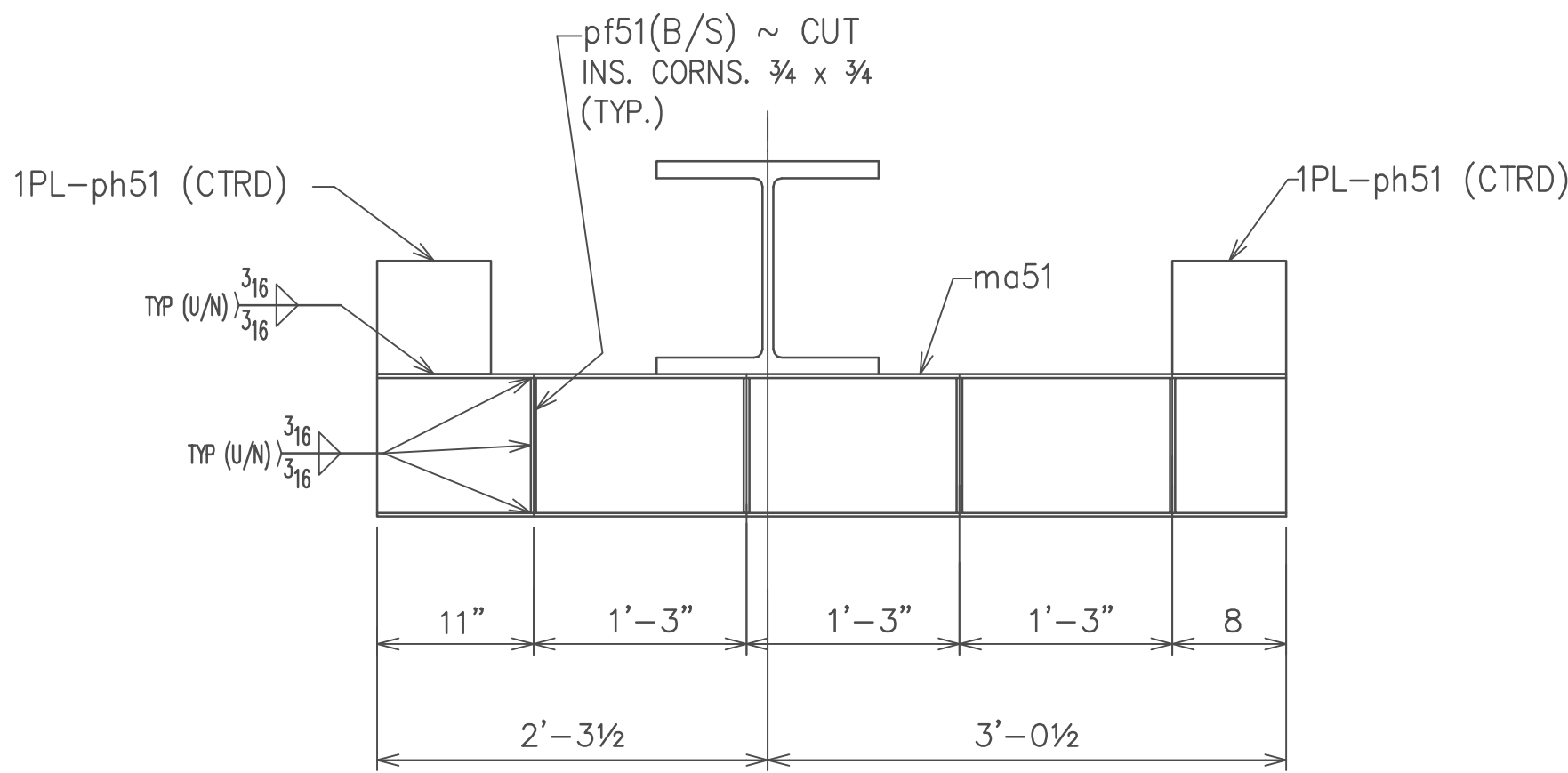
SECTION D
