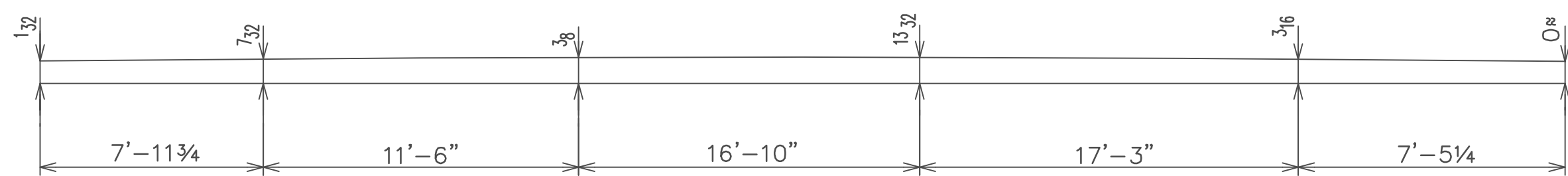
CAMBER DIAGRAM
